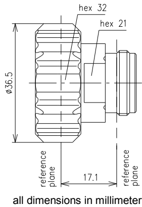
all dimensions in millimeter
