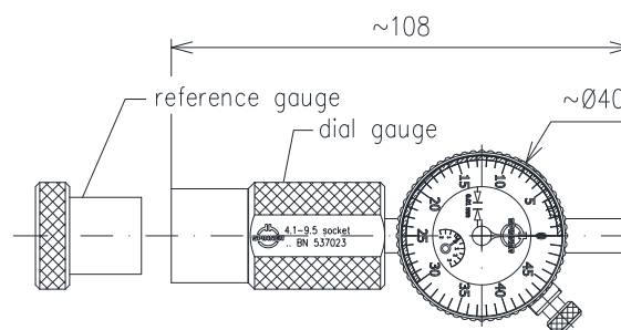
all dimensions in millimeters
