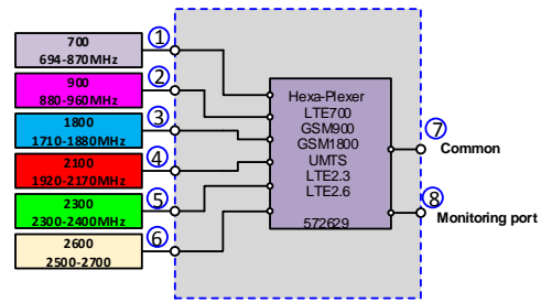
Block Diagram
