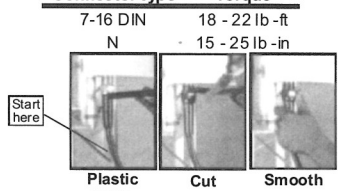
Connector coupling
