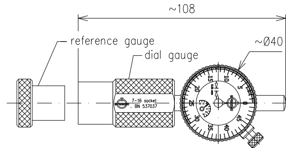
all dimensions in millimeters
