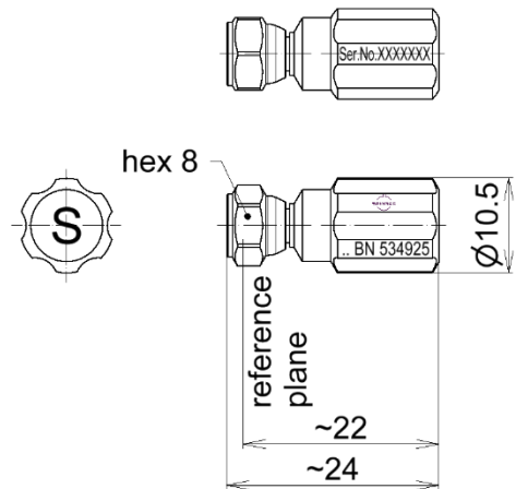
all dimensions in millimeter
